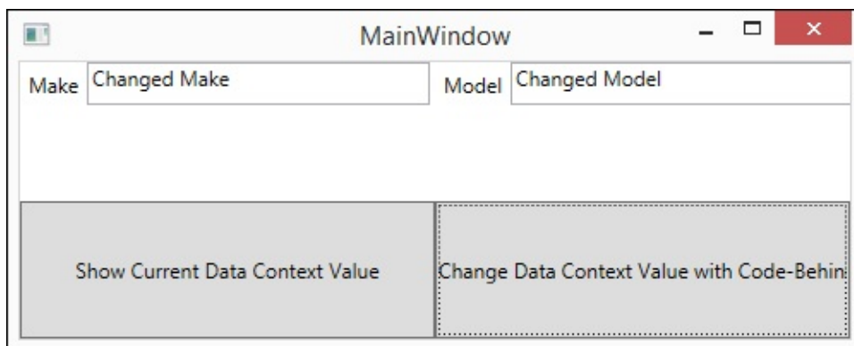
FIGURE 3-3: Two-way data binding with INotifyPropertyChanged .
