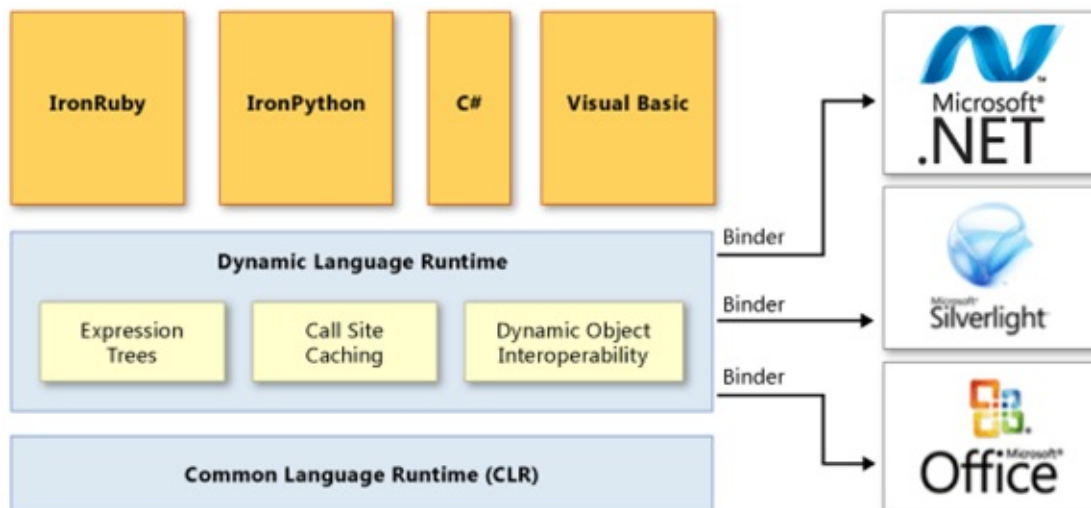
FIGURE 6-1: The Dynamic Language Runtime.
