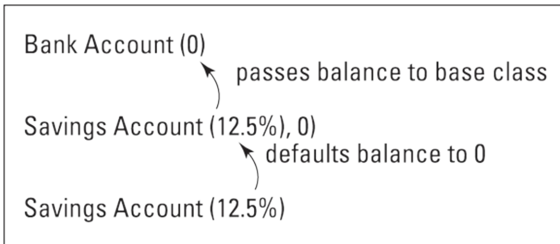
FIGURE 6-1: The path for constructing an object using the default constructor.
