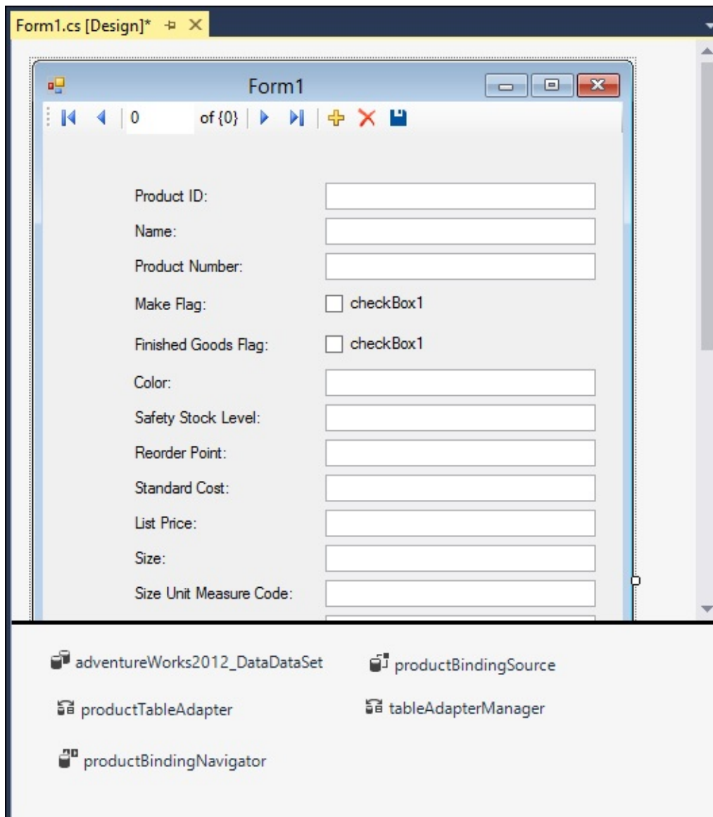
FIGURE 2-10: Creating a Parts Detail data form.
