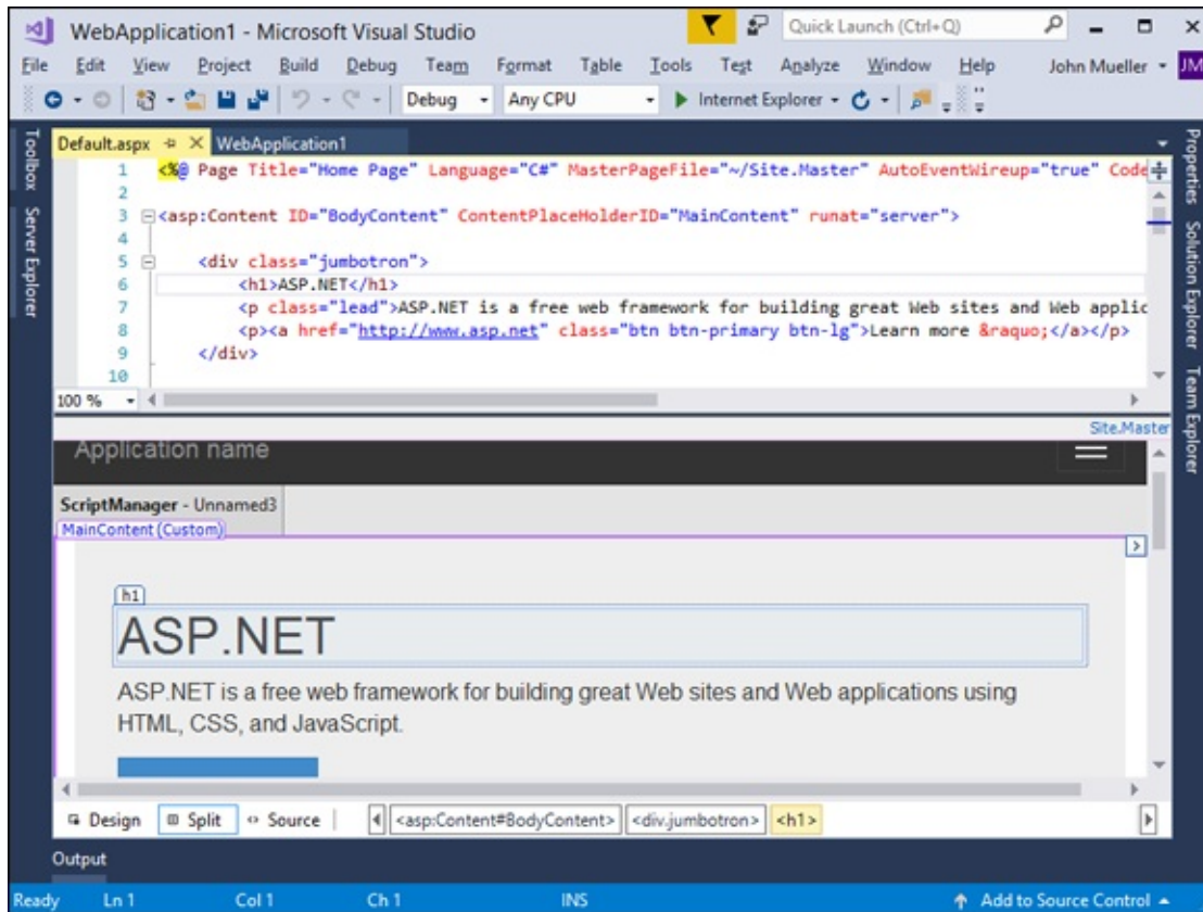
FIGURE 2-3: Back-end code used with web projects.
