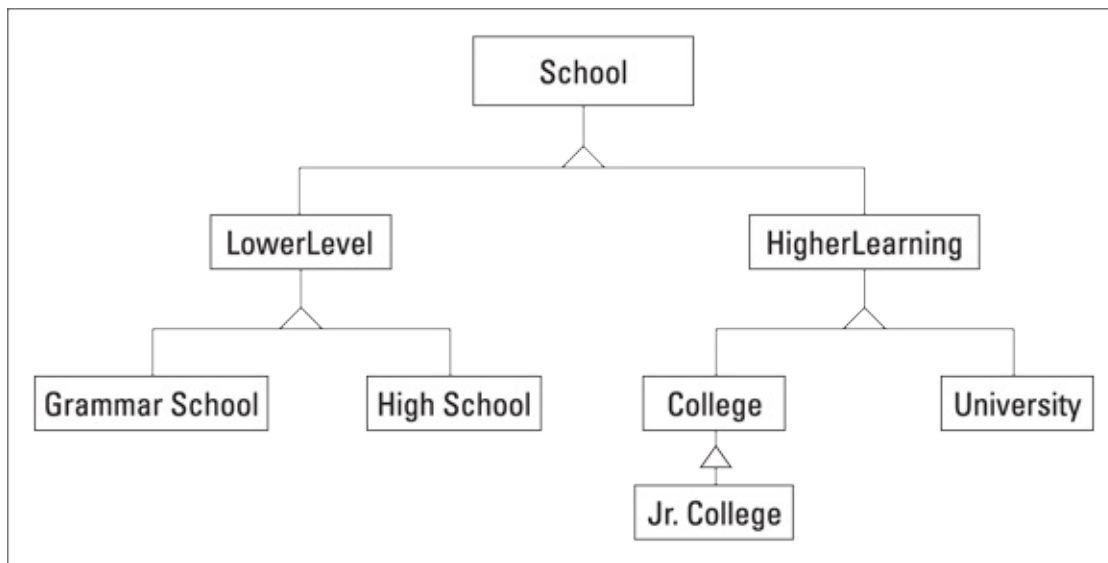
FIGURE 7-4: Class factoring usually results in added layers of inheritance hierarchy.
