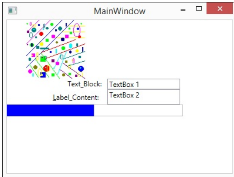
FIGURE 2-14: Display-only controls.
