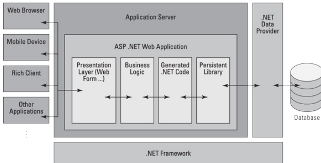
FIGURE 1-2: ASP.NET deconstructed.
