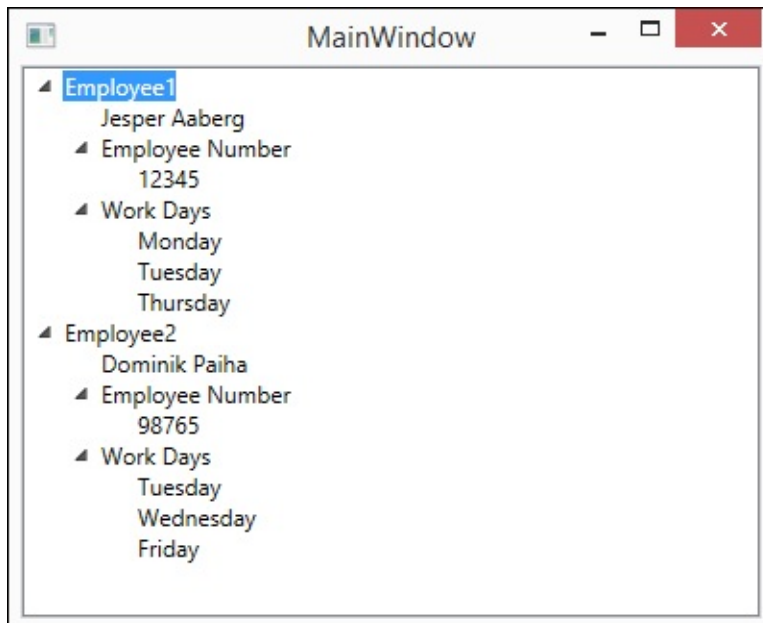
FIGURE 2-17: The TreeView.
