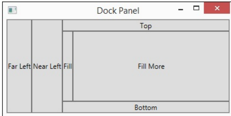
FIGURE 2-5: Dock Panel.
