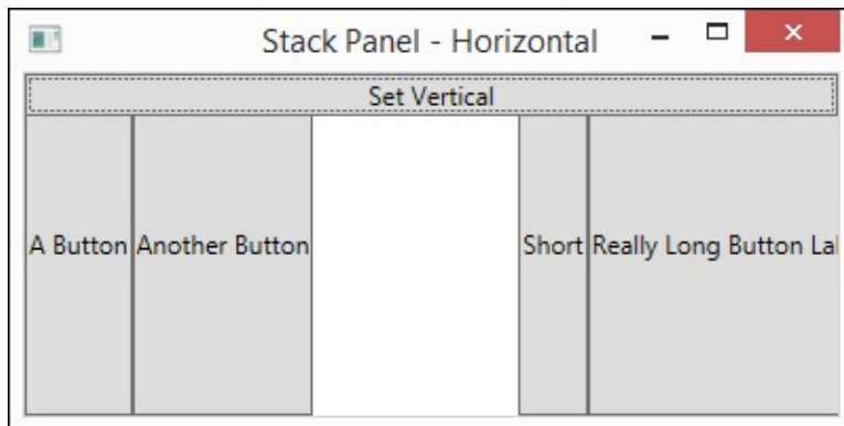
FIGURE 2-2: Horizontal.
