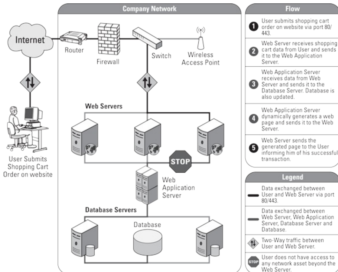
FIGURE 1-1: The web application process.
