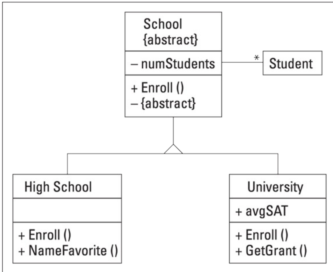
FIGURE 7-3: Base both HighSchool and University on a common School class.
