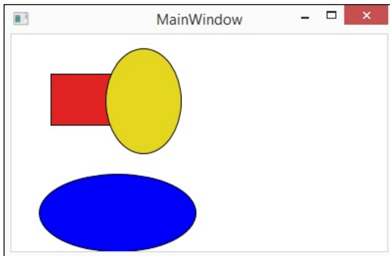
FIGURE 2-6: Canvas sample.
