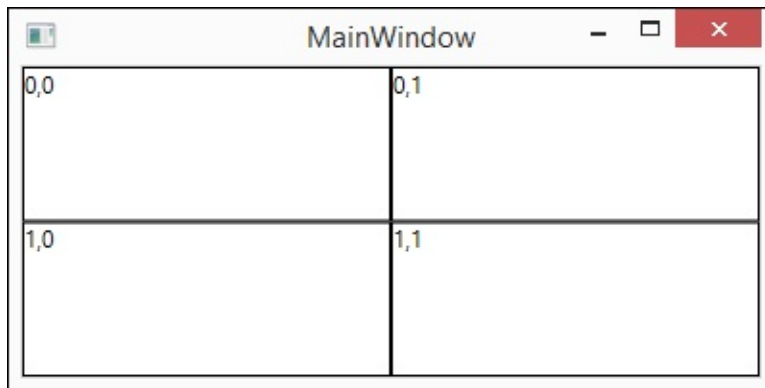
FIGURE 2-7: Uniform Grid.
