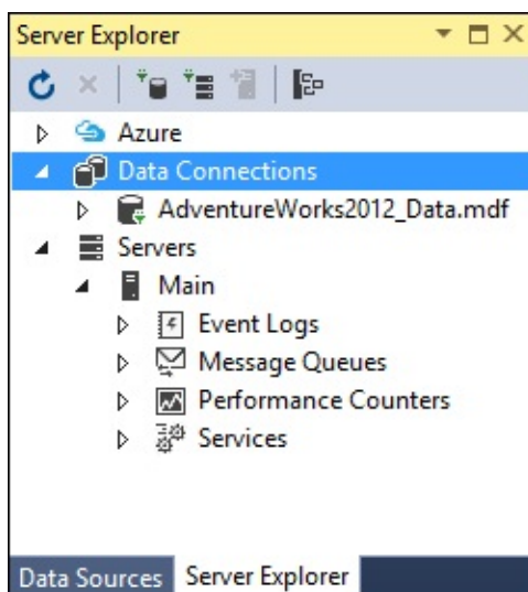
FIGURE 2-9: Server Explorer.
