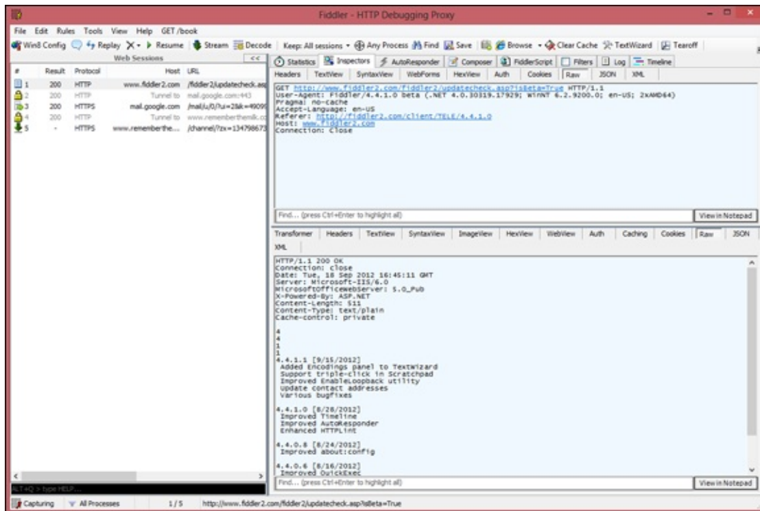
FIGURE 1-4: Fiddler.
